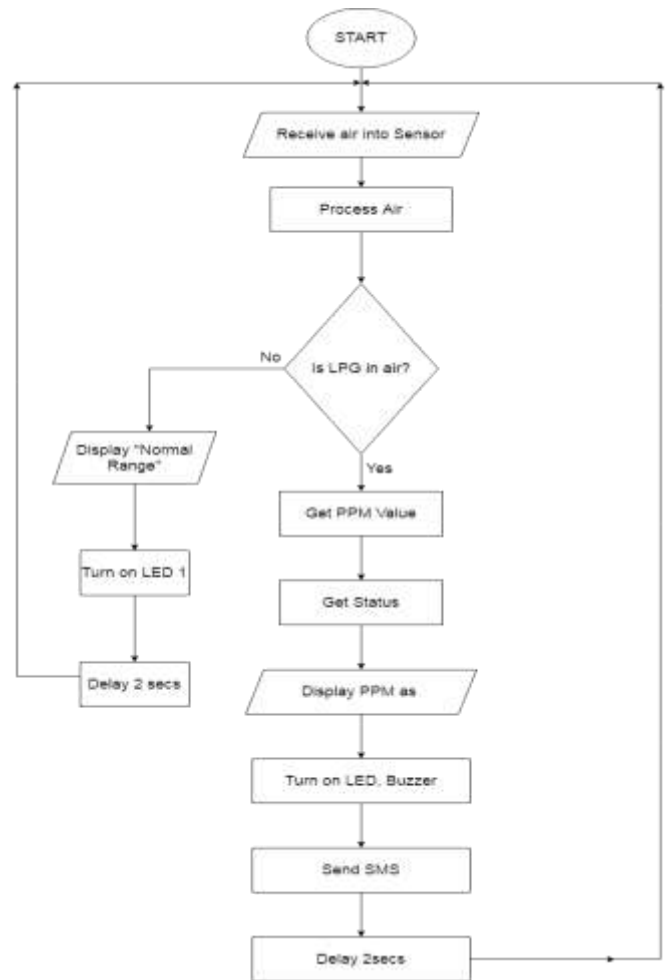
Figure 17: System Flowchart Diagram
